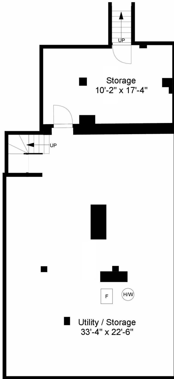
Basement Plan Ceiling Height = 6'-0"
